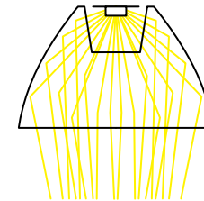
beam path TIR-lens
